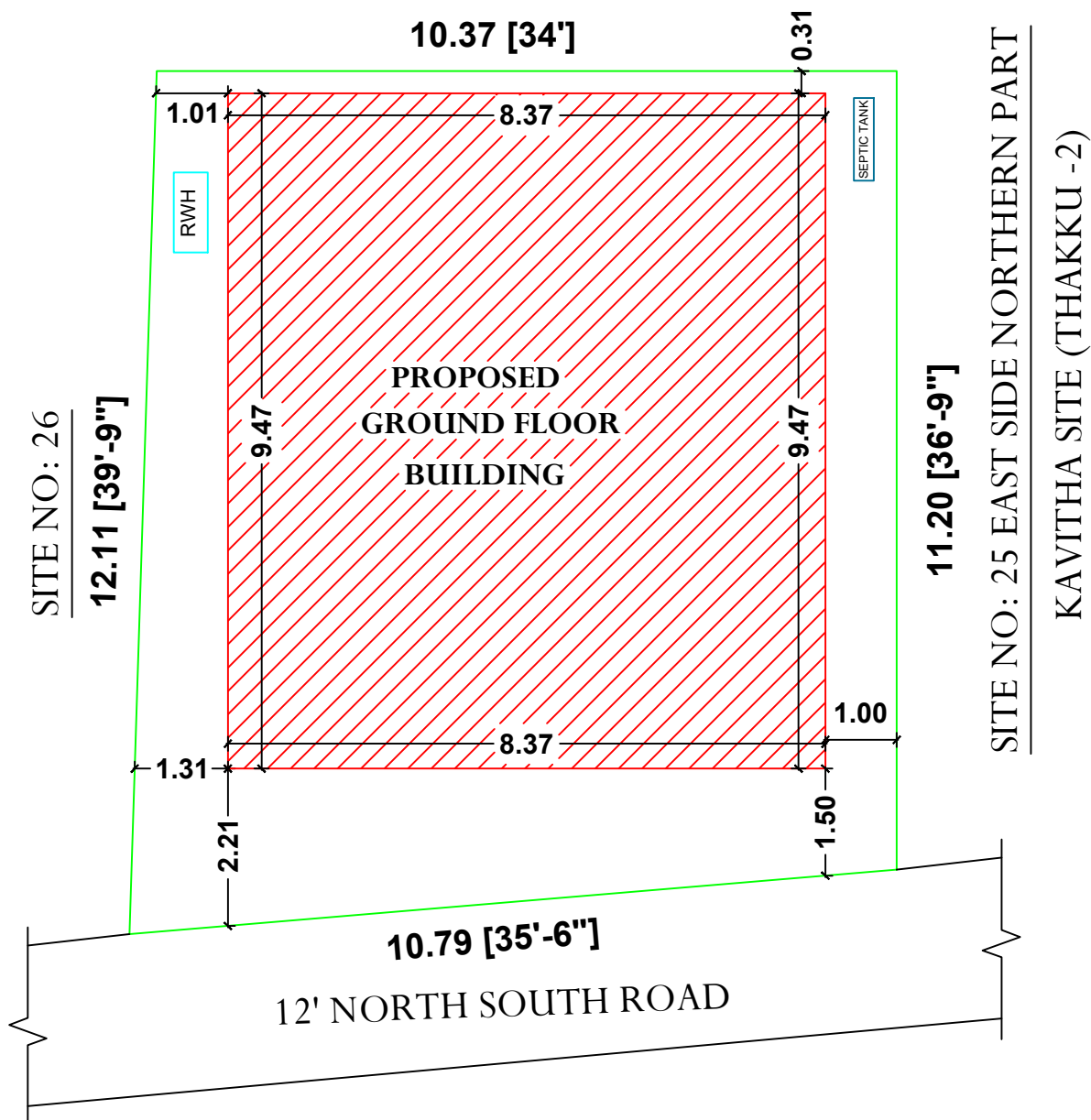
SITE PLAN
