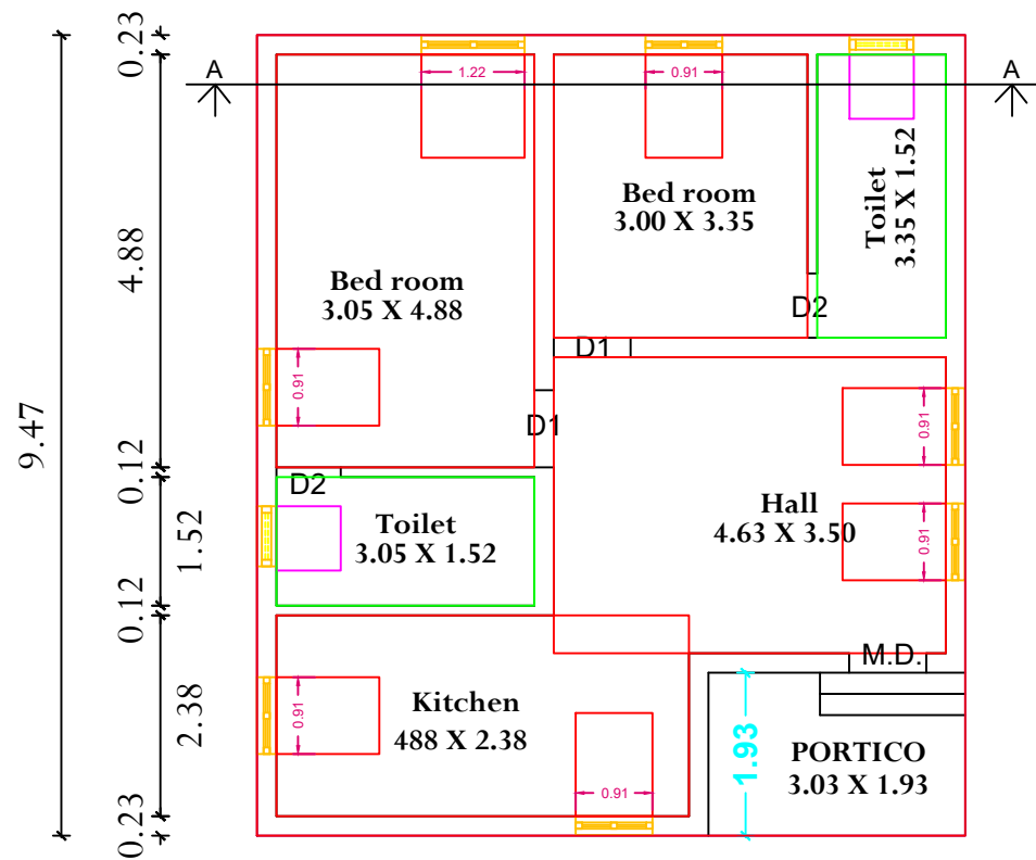
2D FLOOR PLAN
