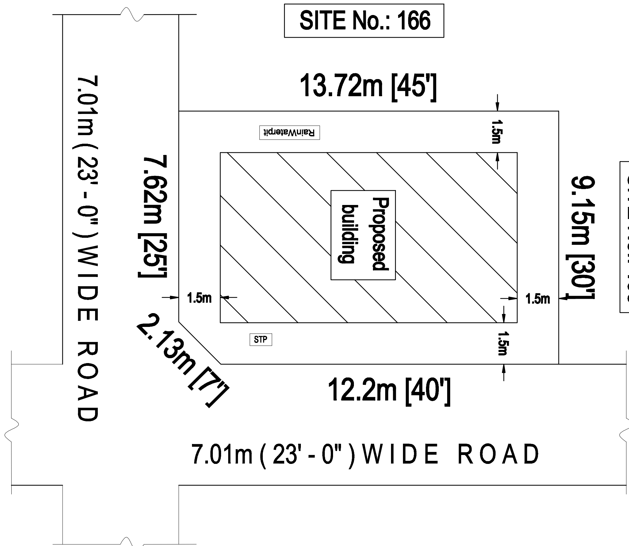
SITE PLAN
