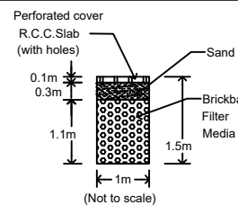
RAIN WATER HARVESTING RECHARGE TRENCH SECTION
