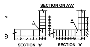
TYPICAL DETAILS OF PROVIDING VERTICAL STEEL BARS IN BRICK MASONRY
