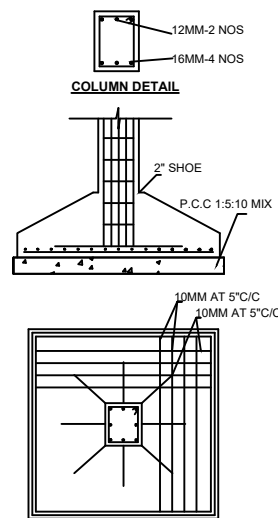
FOOTING DETAIL SCALE: NTS
