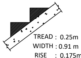
STAIRCASE DETAIL:
