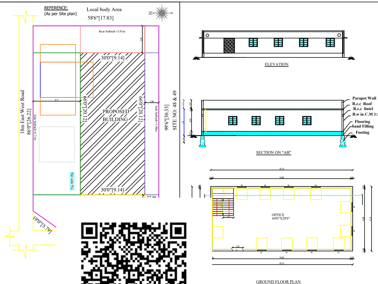
SITE PLAN
