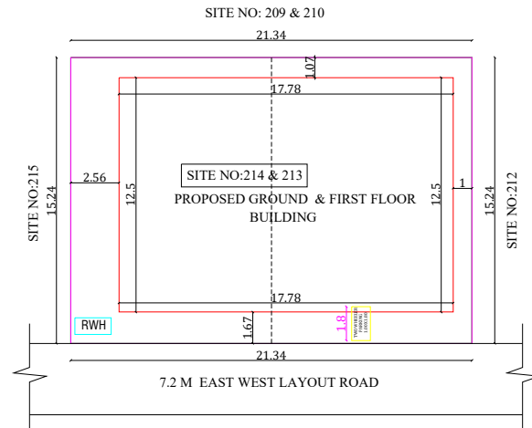
SITE PLAN
