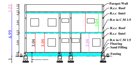
SECTION A - B
