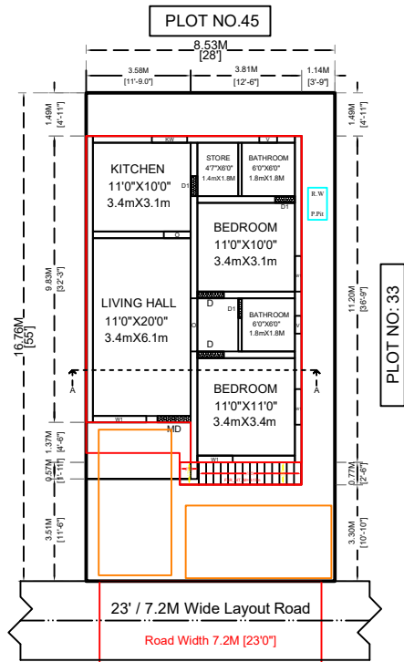
SITE CUM EXISTING GROUND FLOOR PLAN
