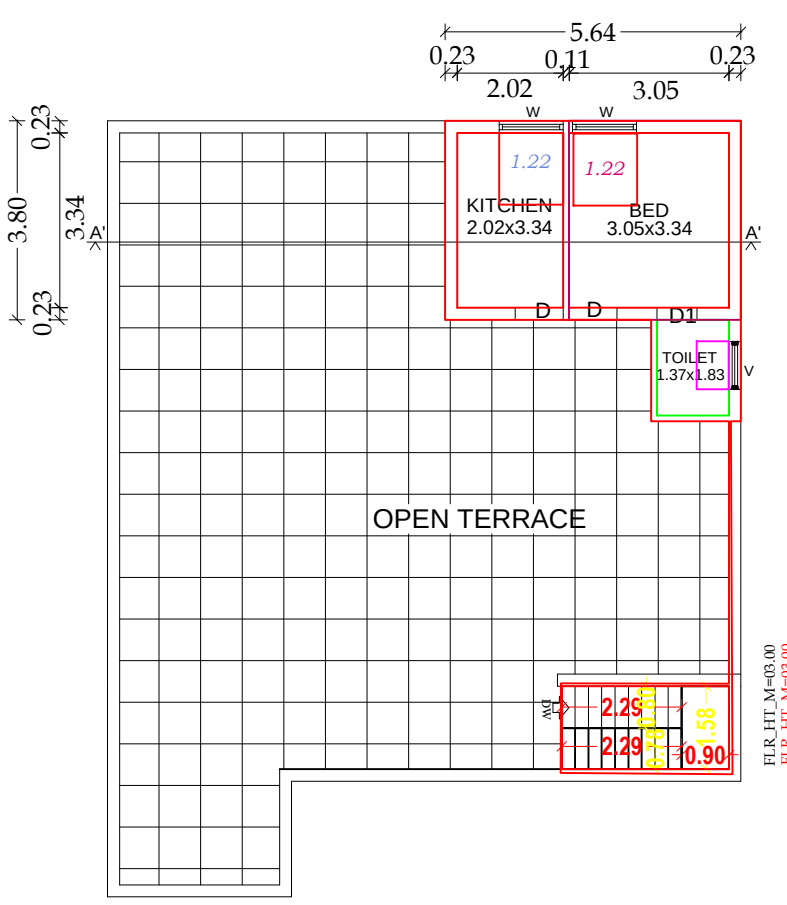
PRO. ADD. SECOND FLOOR PLAN
