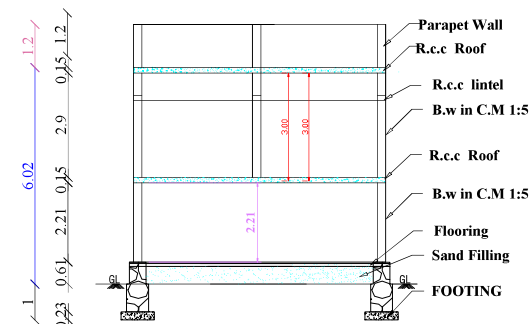
CROSS SECTION AT A-A
