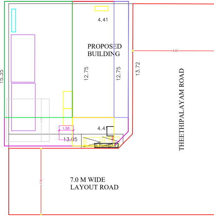
SITE PLAN
