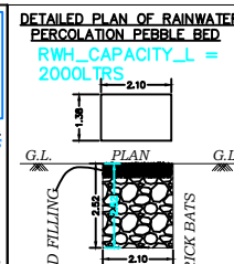
Section Not to Scale
