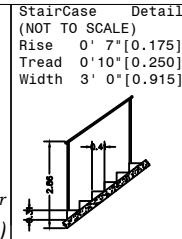
StairCase Detail
