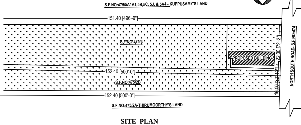
SITE PLAN
