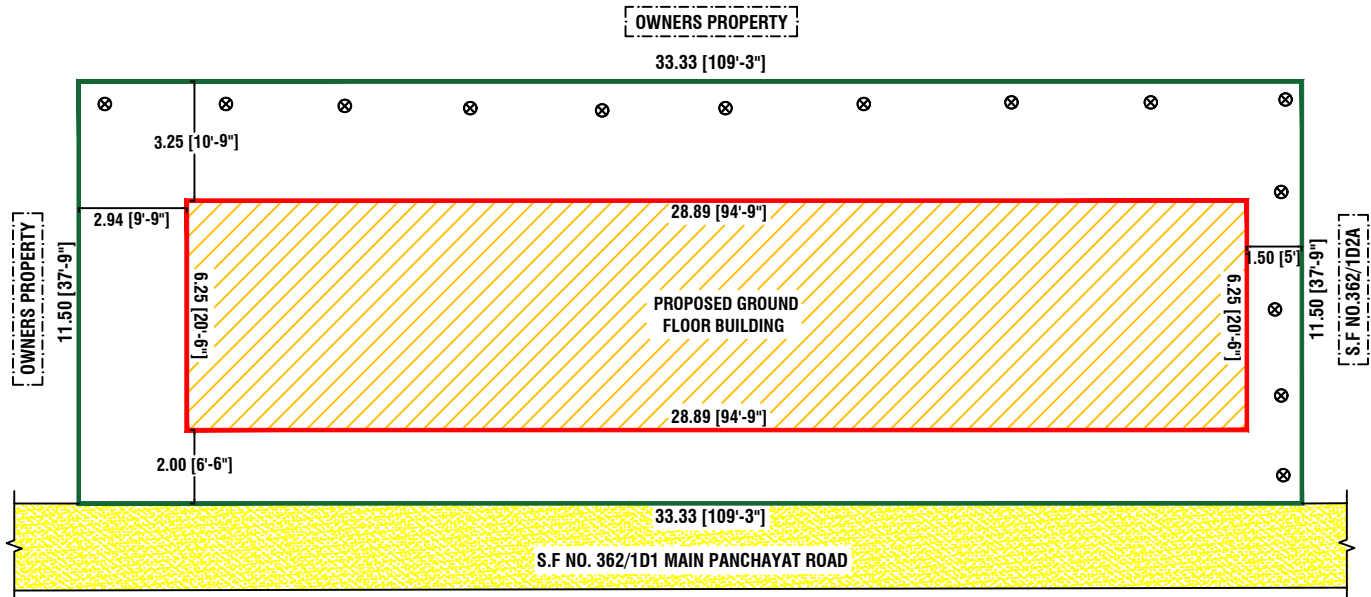
SITE PLAN
