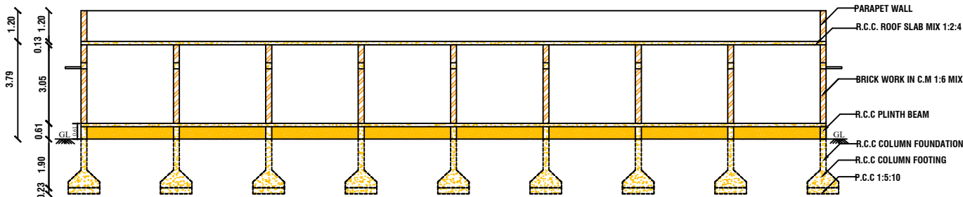
CROSS SECTION AT A-A
