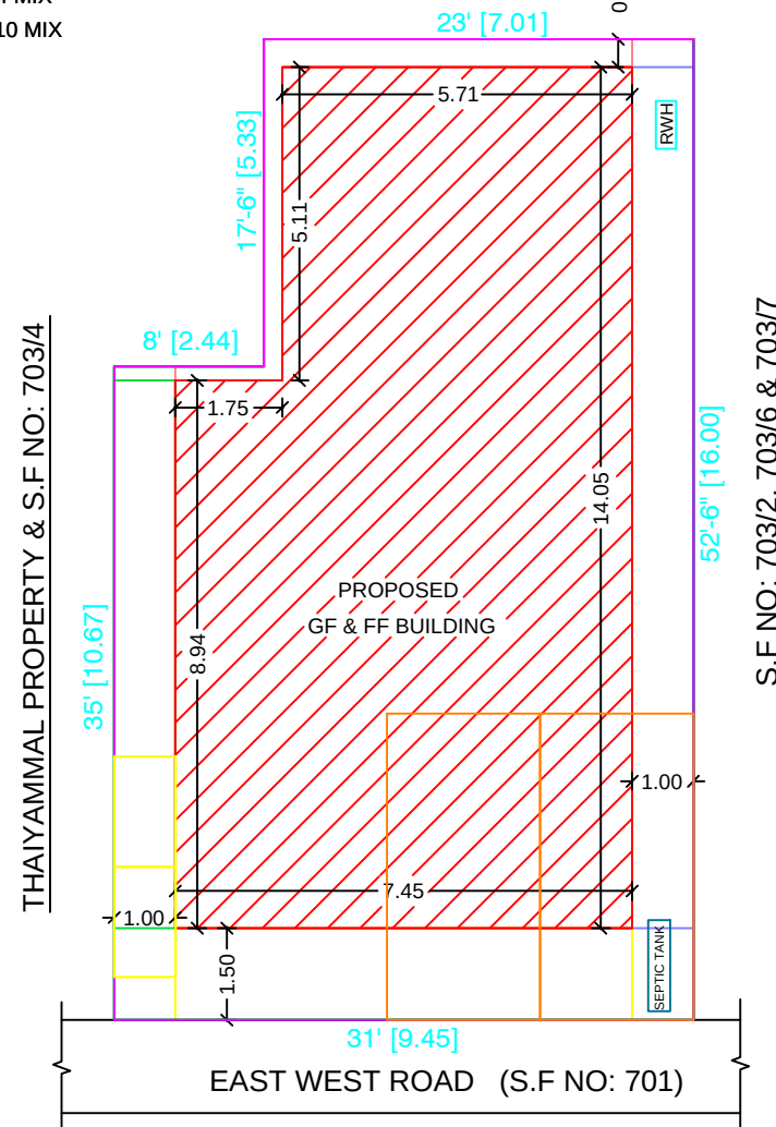
SITE PLAN
