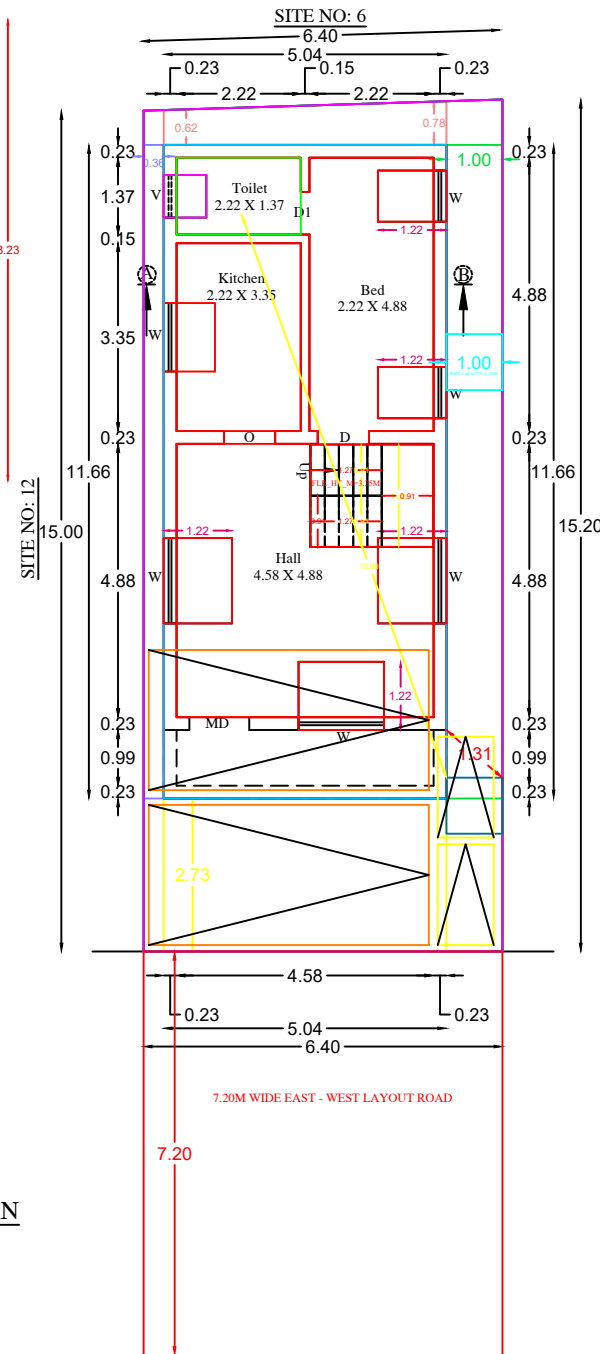
SITE PLAN & PROPOSED GROUND FLOOR PLAN
