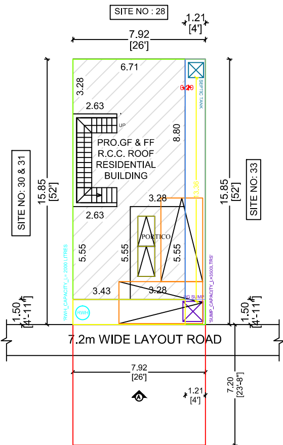
SITE PLAN
