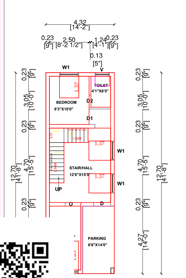
1 Floor Plan
