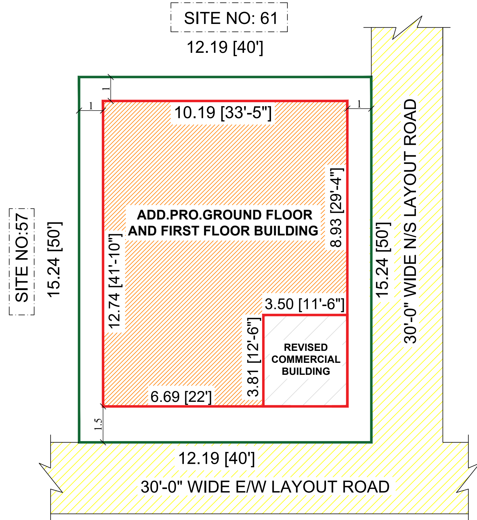
SITE PLAN
