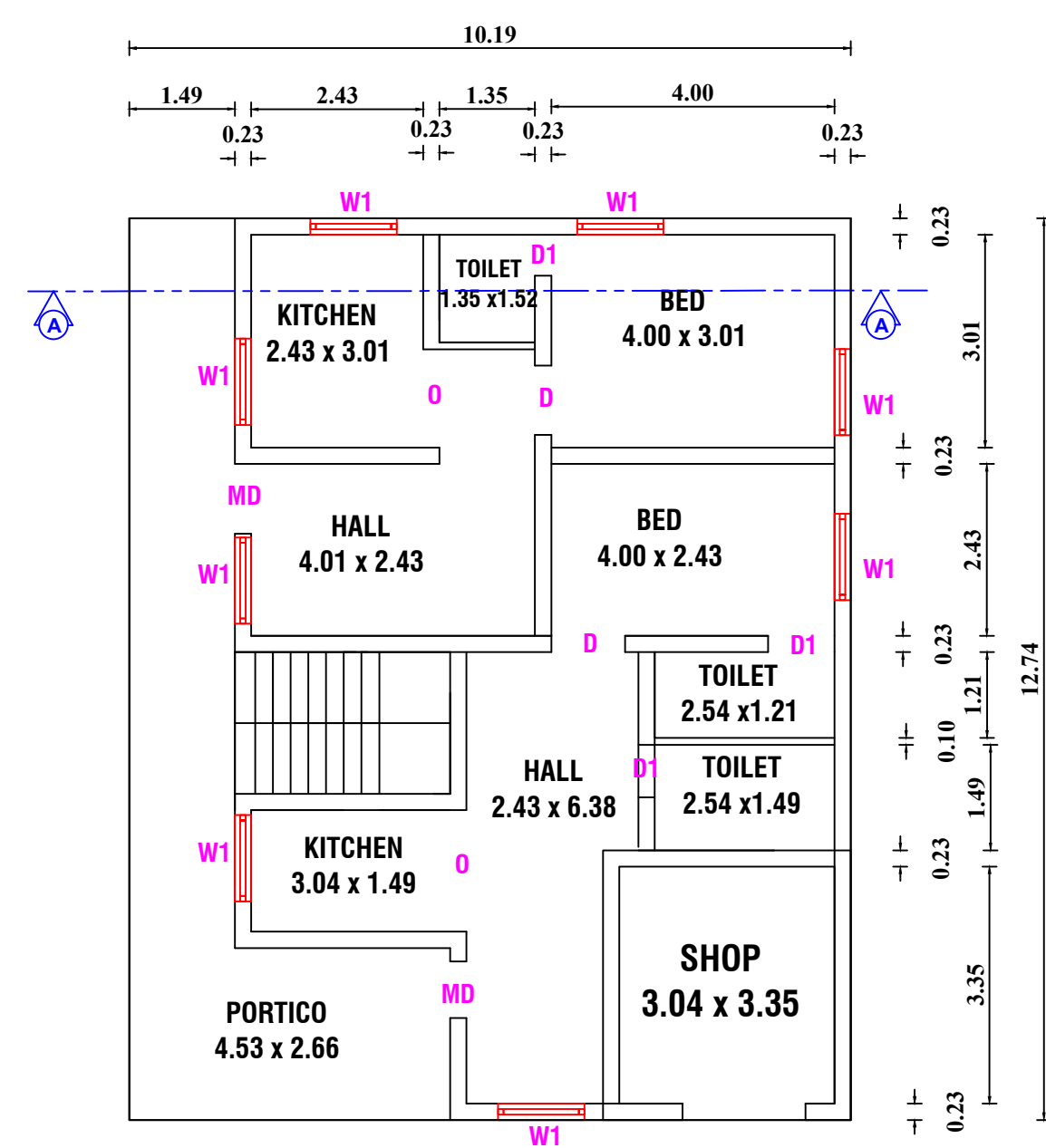
REVISED & ADD.PRO.GROUND FLOOR PLAN
