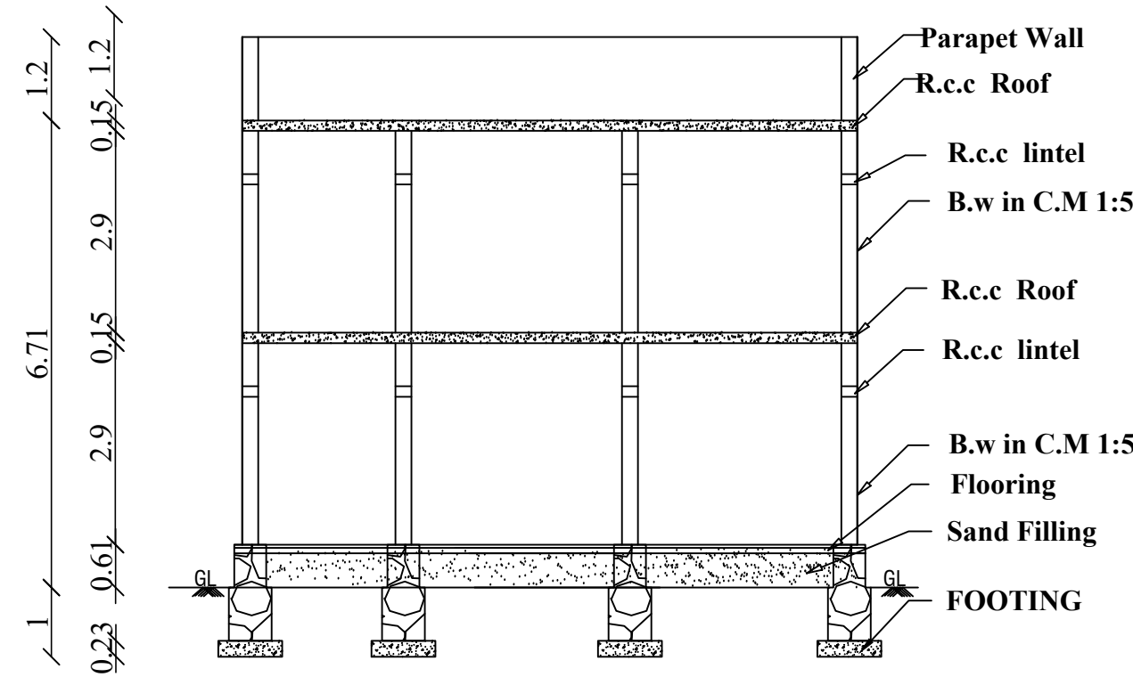
CROSS SECTION AT A-A
