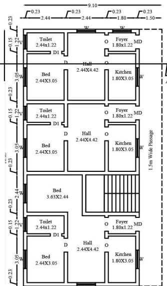
PROPOSED SECOND FLOOR PLAN
