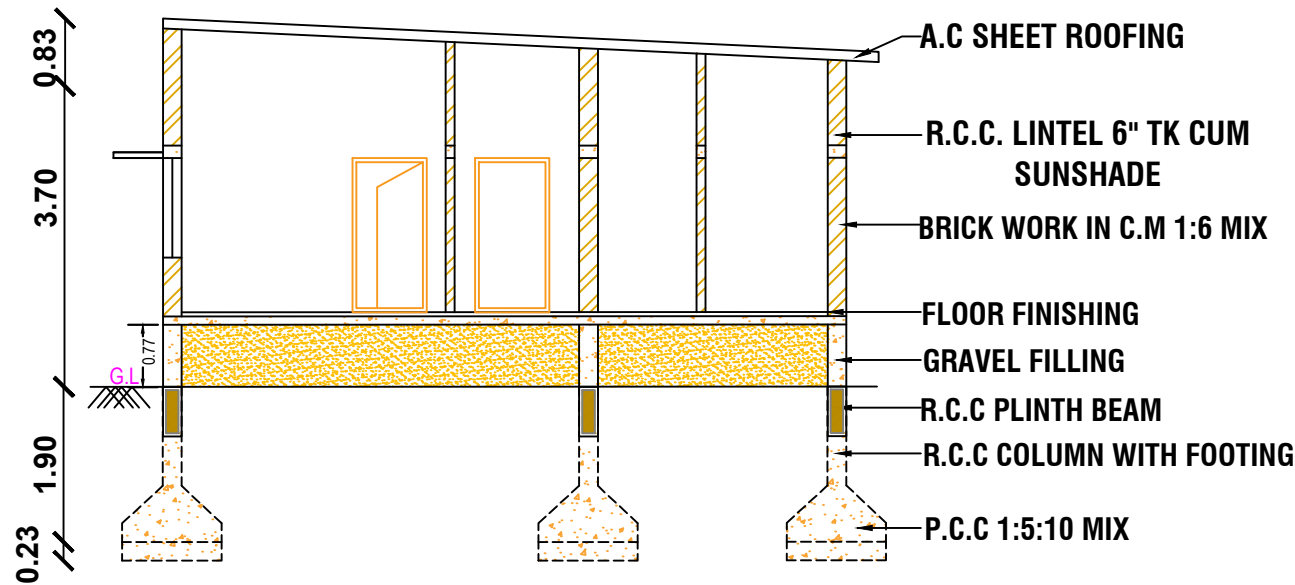
CROSS SECTION AT A-A
