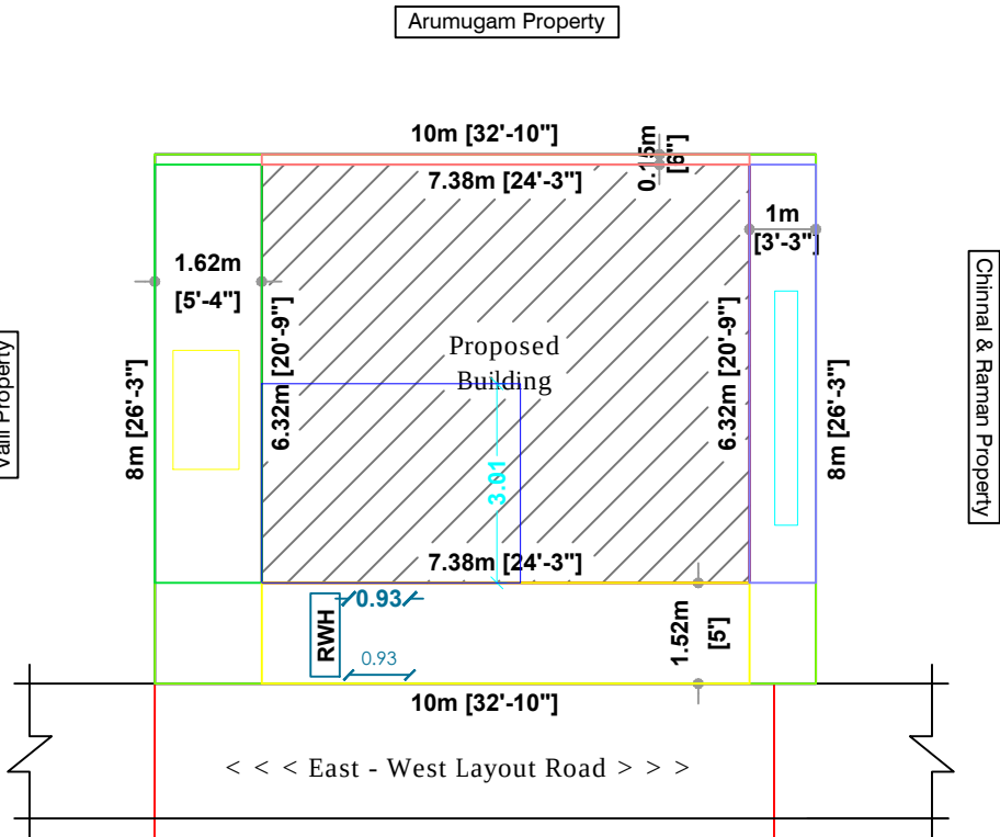
SITE PLAN
