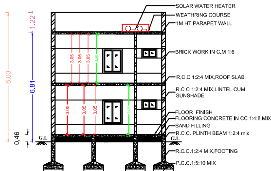
SECTION AT ( B - B )
