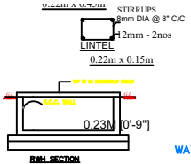
COLUMN POST DETAILS
