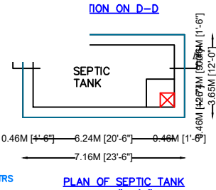
PLAN OF SEPTIC TANK SCALE 1"=2'-0"
