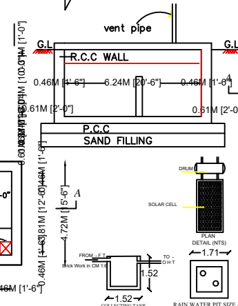
SUMP DETAIL SCALE 1"=4'-0"
