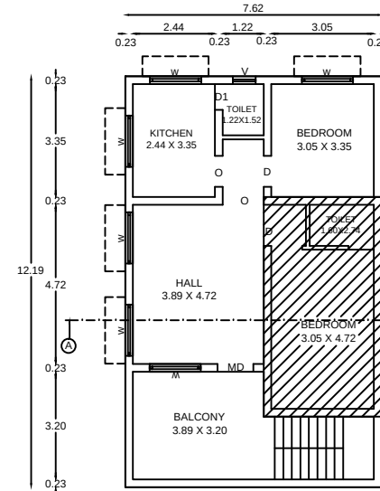
ADD. PROPOSED FIRST FLOOR
