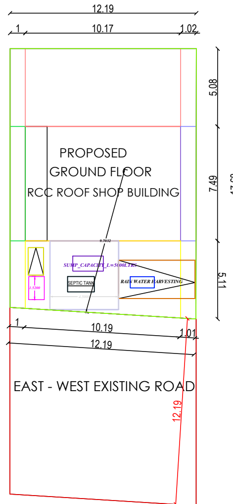
SITE PLAN
