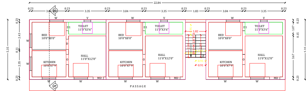
EX & ADD. GROUND FLOOR PLAN
