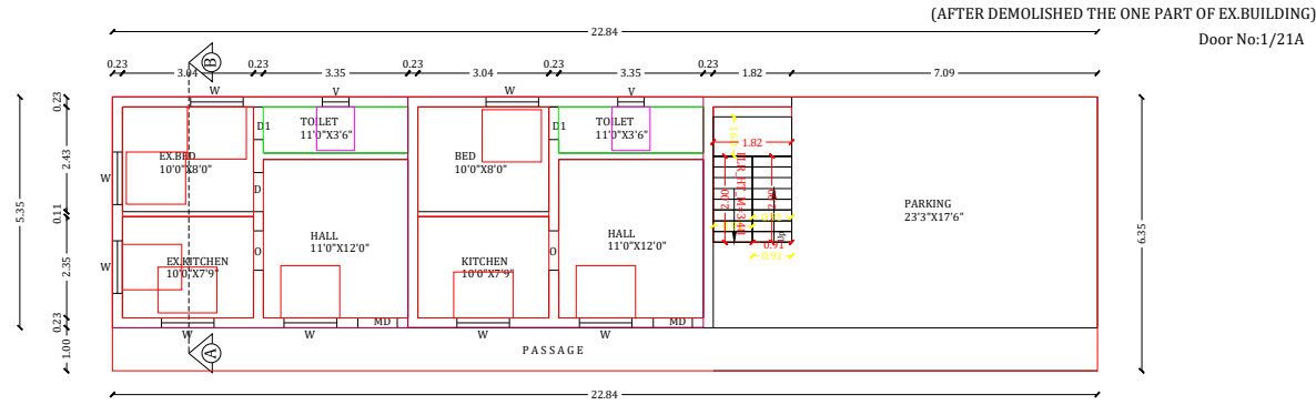
EX & ADD. GROUND FLOOR PLAN
