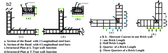
Figure - 2 : Reinforcement and Bending Details of Seismic Bands.
