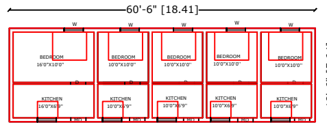
PROPOSED GROUND FLOOR PLAN
