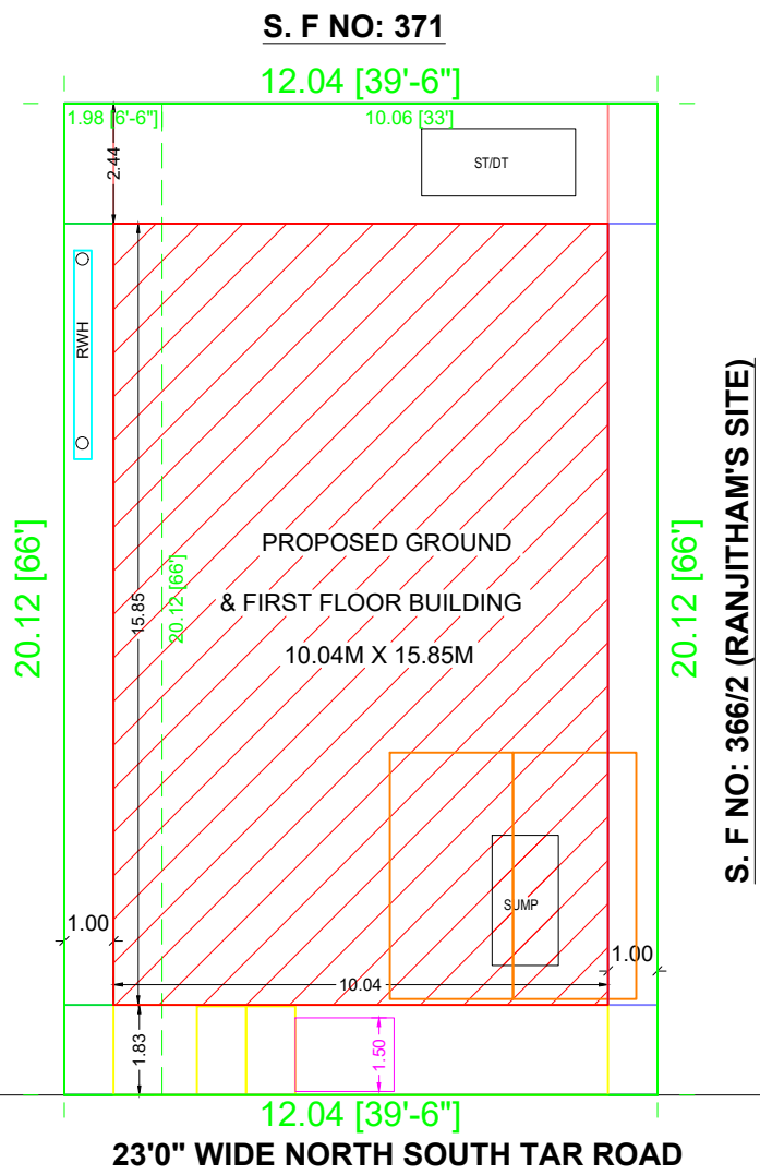
SITE PLAN
