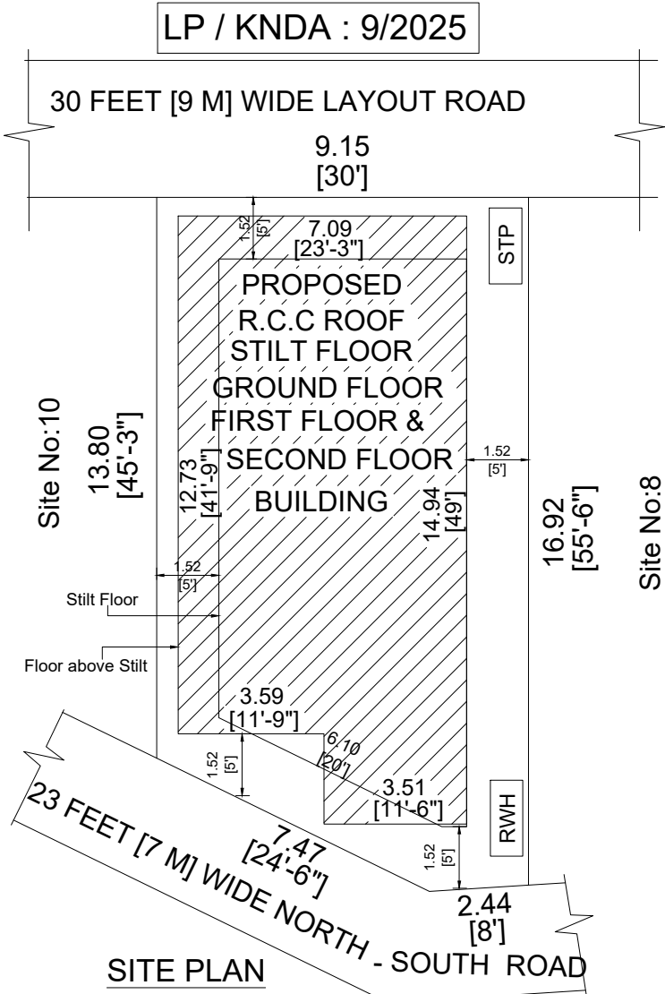
SITE PLAN
