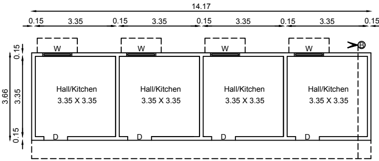
LABOUR SHED PLAN
