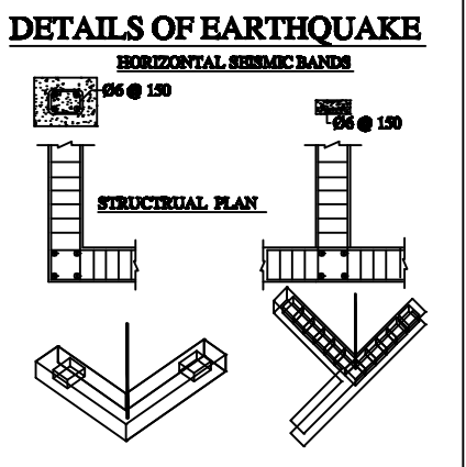
DETAILS OF EARTHQUAKE RESISTANT CONSTRUCTION
