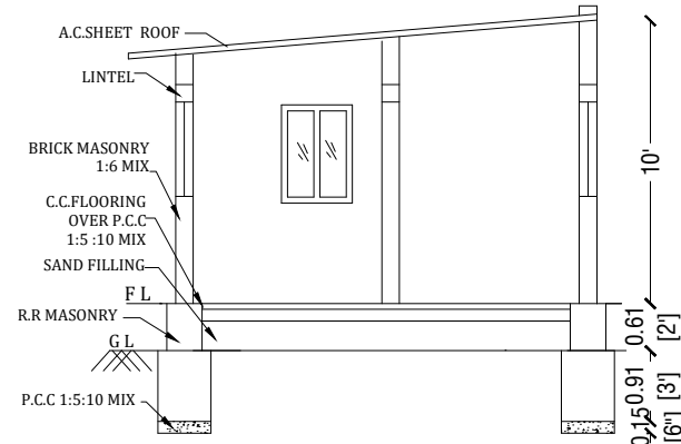
SECTION AB
