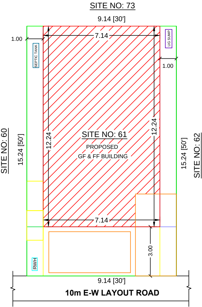
SITE PLAN
