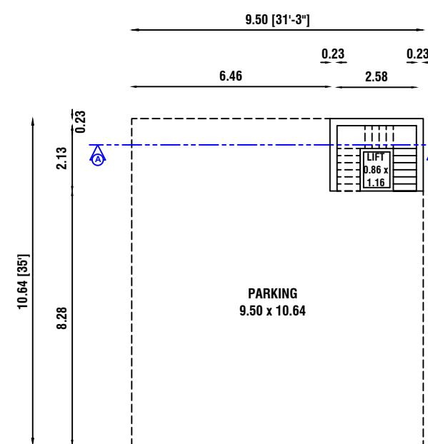
STILT FLOOR PLAN
