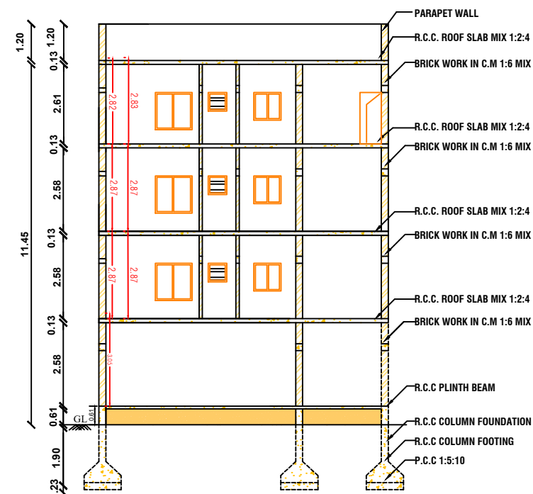
CROSS SECTION AT A-A
