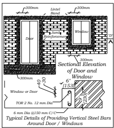
Sectional Elevation of Door and Window
