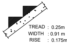
STAIRCASE DETAIL:
