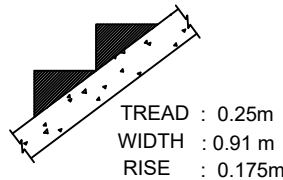
STAIRCASE DETAIL:
