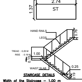
STAIRCASE DETAILS
