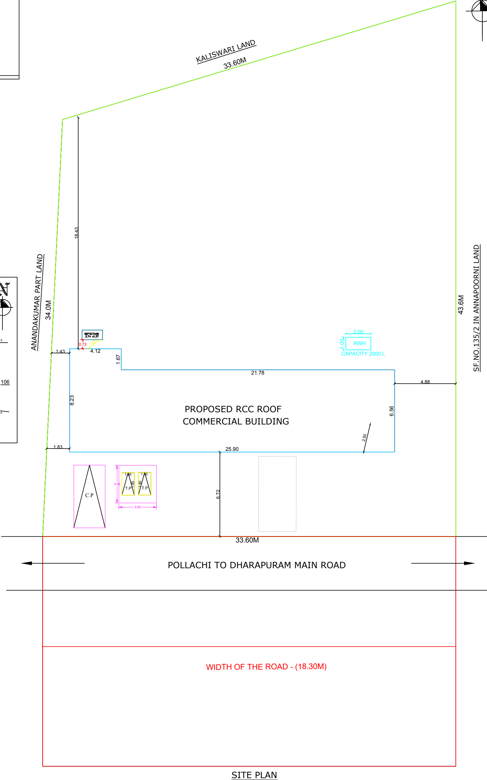
SITE PLAN
