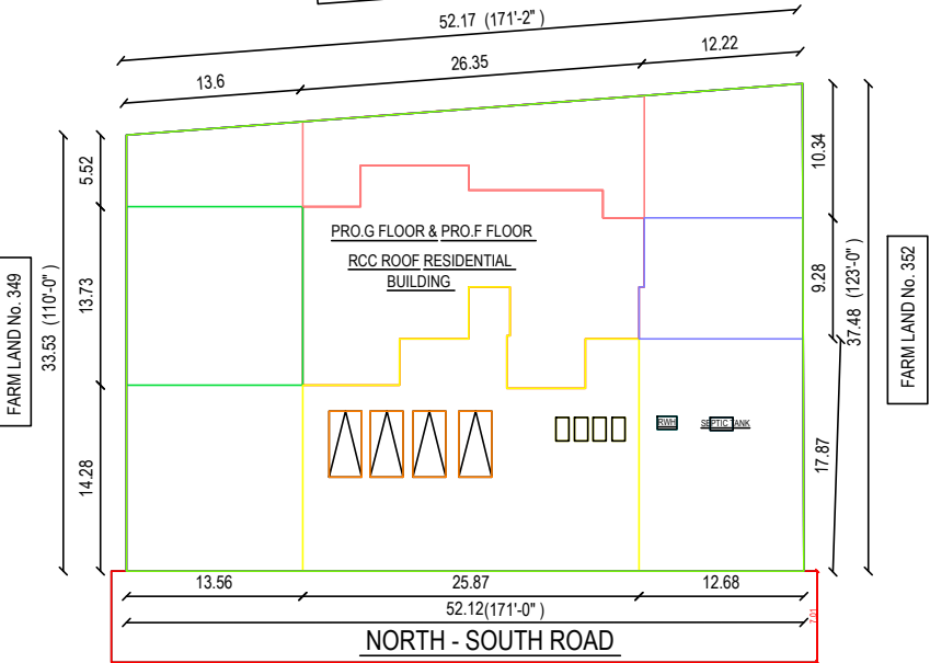
SITE PLAN
