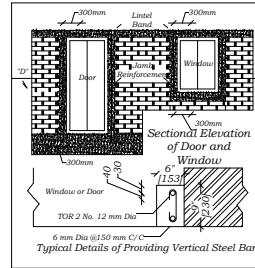
Sectional Elevation of Door and Window
