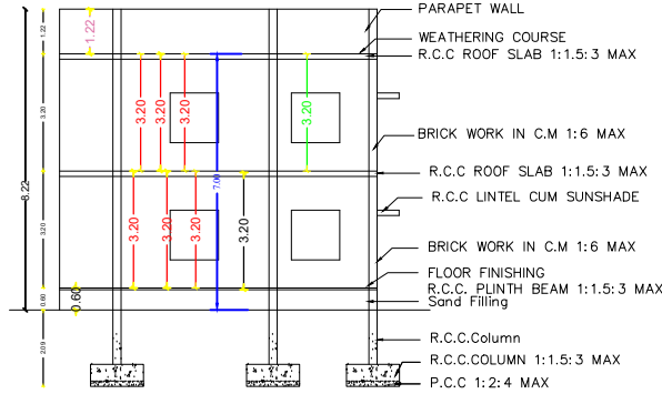
SECTION
