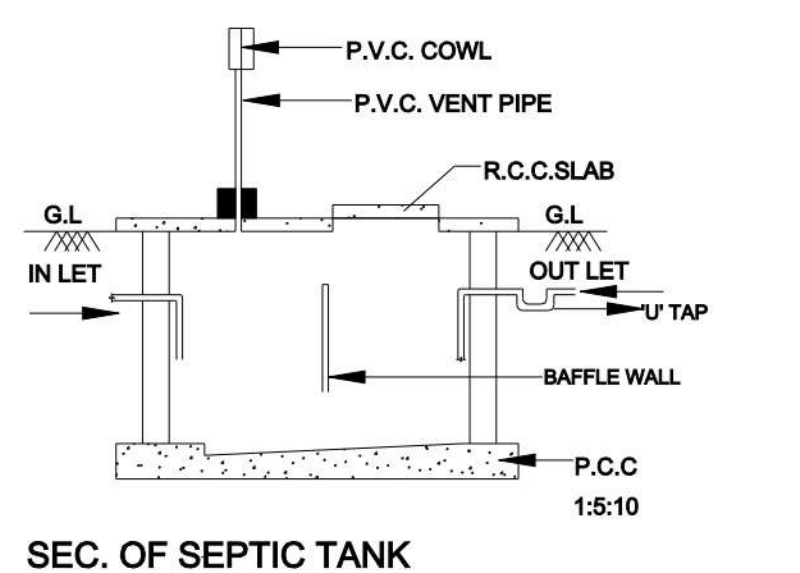
SEC. OF SEPTIC TANK
