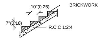
STAIRCASE WAIST SLAB
