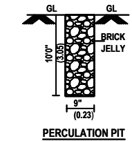
PERCOLATION PIT
