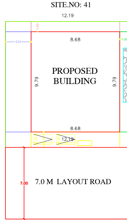
SITE PLAN
