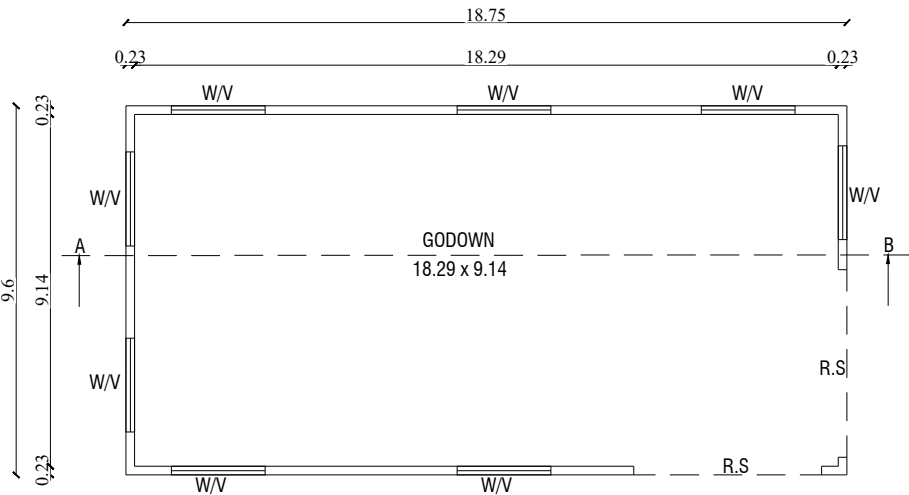
PRO.GROUND FLOOR PLAN
