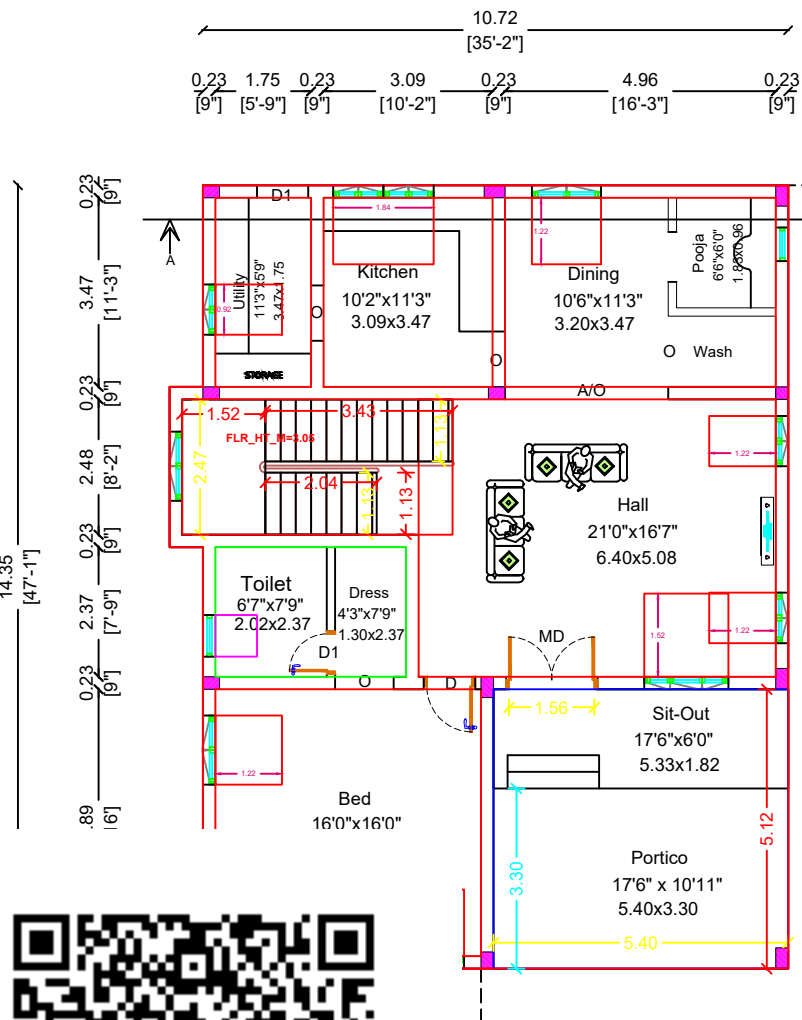
ID FLOOR PLAN
