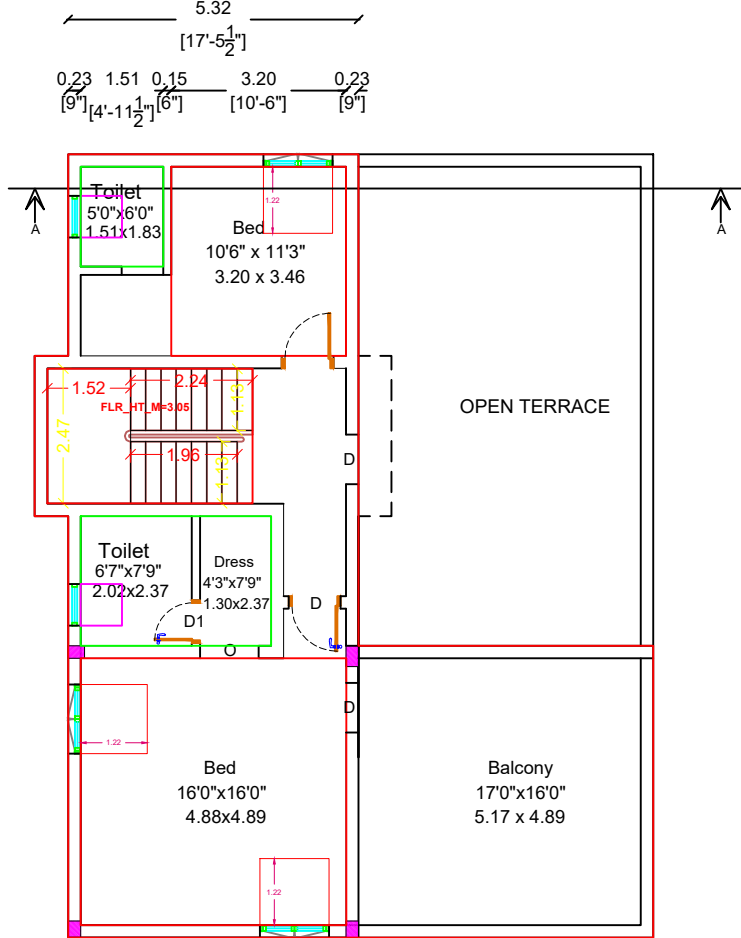
ADD. PRO. FIRST FLOOR PLAN
