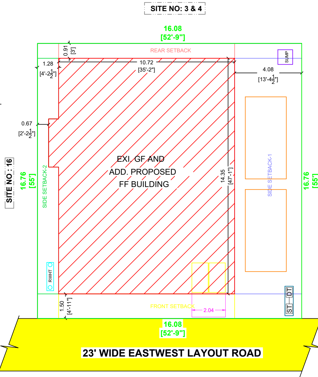
SITE PLAN
