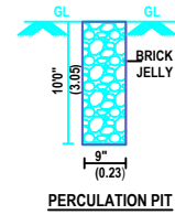
PERCOLATION PIT
