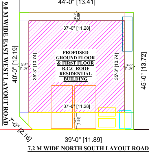
SITE PLAN
