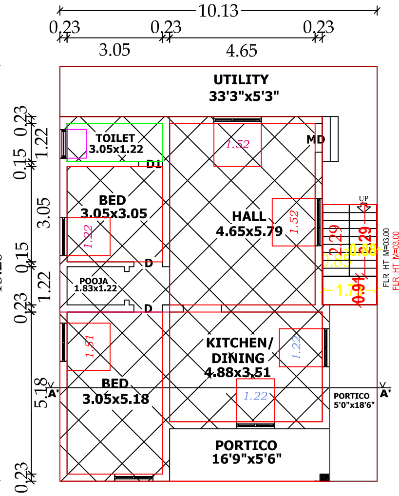
EXG. AND PRO. ADD. GROUND FLOOR PLAN
