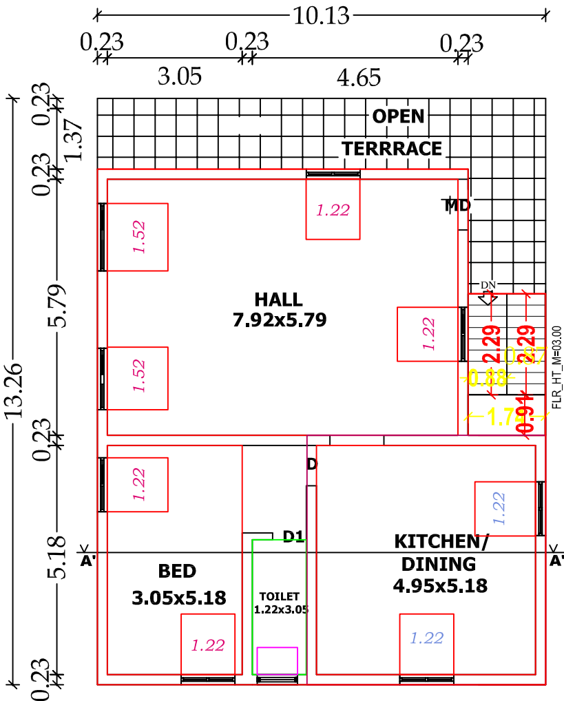
PRO. ADD. FIRST FLOOR PLAN
