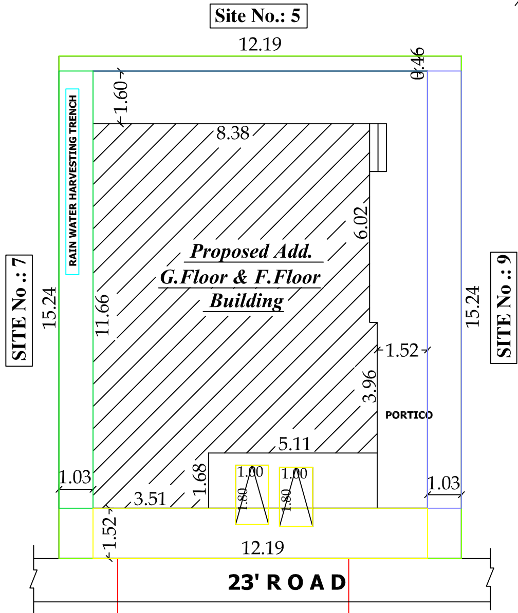
SITE PLAN
