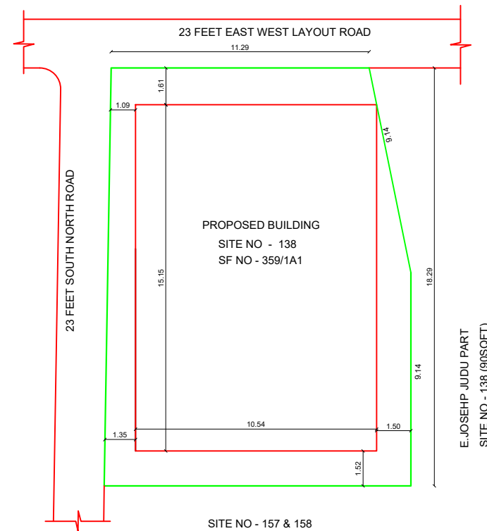
SITE PLAN
