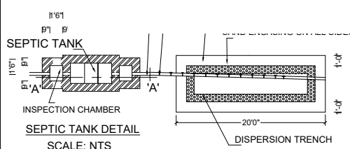
SEPTIC TANK DETAIL SCALE: NTS
