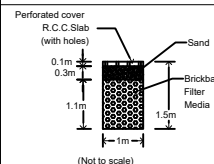
RAIN WATER HARVESTING RECHARGE TRENCH SECTION
