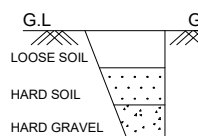
TRIAL PIT SCALE: NTS
